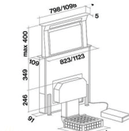
Filtering version (Slim motor) with Carbon.Zeo underbase filter (KACL.930)
