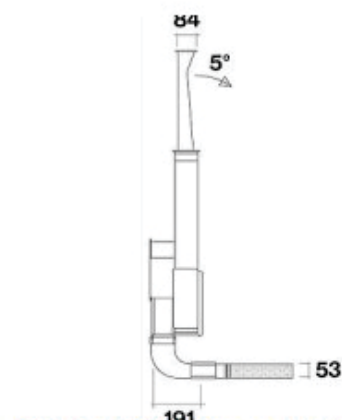
Side view, Slim motor on the back, Under base slim filter KACL.951 (h60)
