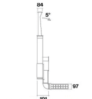
Side view, Slim motor on the front
