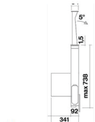
Side view, motor on the back
