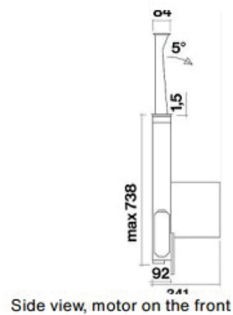
Ducted version (onboard 950 m3/h motor)
